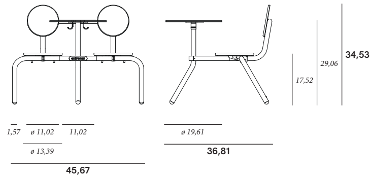
Bistrou with purse hanger & stacking spacer
