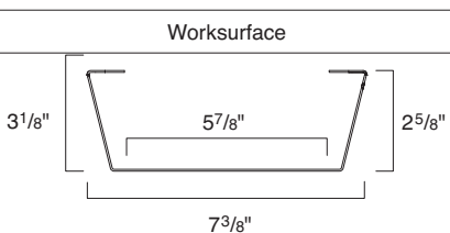
Cable tray side view
