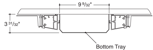
Bottom Tray
