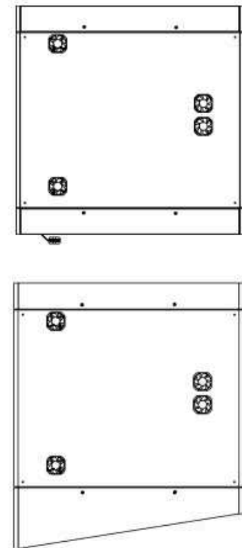
Plan view 4 x ventilation fans. Top: no kink Bottom: with kink
