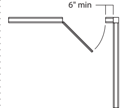
Strike jamb at two-way 90° junction Minimum 6" from junction Acceptable
