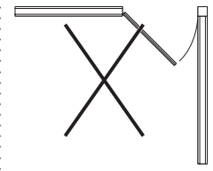
Strike jamb at two-way 90° junction Swing to inside of junction Not Acceptable
