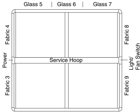
Air25 configuration
