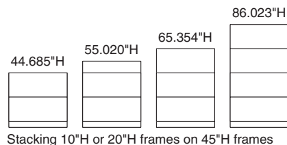
Stacking 10"H or 20"H frames on 45"H frames
