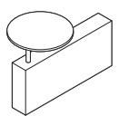
Overall: 28"D 4 1/2"W 15 3/4"H With Tablet: 15 3/4" Dia. and 25 3/8"H
