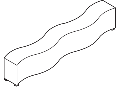
Overall: 19¼"D 97"W 19¼"H Seat Surface: 19"H
