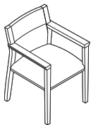
Overall: 22 3 / 4 "D 22 3 / 20 "W 32"H Inside: 19"D 18 1 / 2 "W 14"H Seat: 18"H Arm: 26"H
