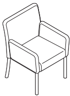
Overall: 22½"D 25¾"W 33½"H Inside: 18½"D 19"W 15½"H Seat: 18½"H Arm: 26½"H
