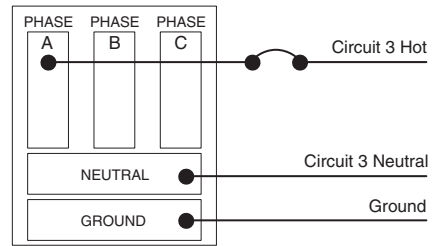
Circuit Panel 2
