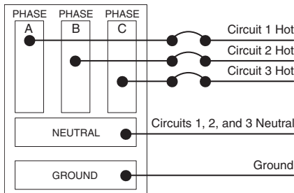
Circuit Panel 2
