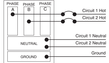
Circuit Panel 1
