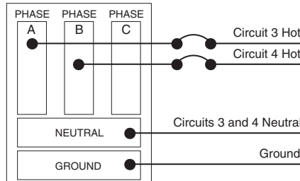
Circuit Panel 2
