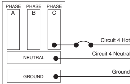
Circuit Panel 2
