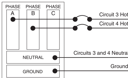
Circuit Panel 2
