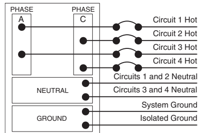
Circuit Panel
