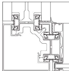
90° inside corner flush skin seal
