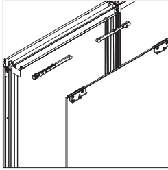
The slider track includes the sliding trolley hardware with close-assist functionality.
