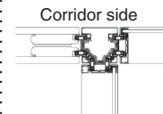
Three-Way junction 90°
