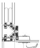
Three-Way 90°
