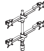
CF Series Dual Static Modular Monitor Arm Assembly with Pole Specifying ▶ Page 187
