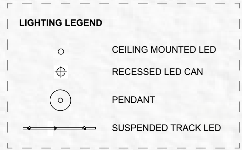
Reflected Ceiling Plan work cafe and workstations
