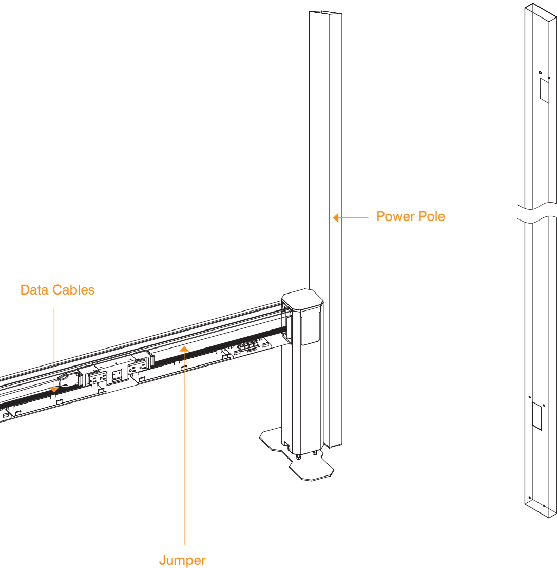
3 Circuit
