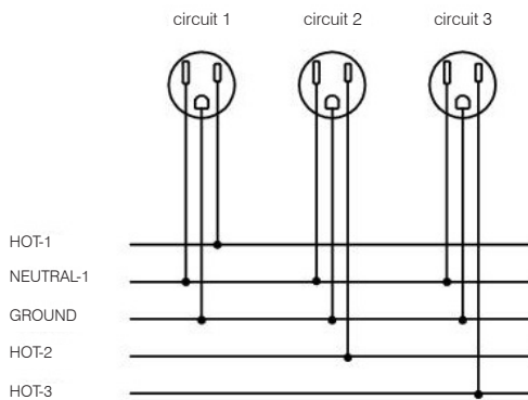
Wire Diagram for 3 Keying
