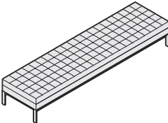
Overall: 26"D 104"W 16½"H
