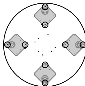
Round Table Top - 36", 42" & 48" Dia POST LEG
