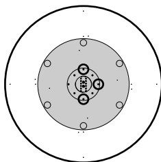
Round Table Top - 36", 24" & 48" Dia. ROUND LEG WITH 5" DIA. COLUMN
