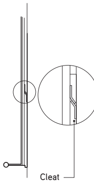
Wall-mount frame
